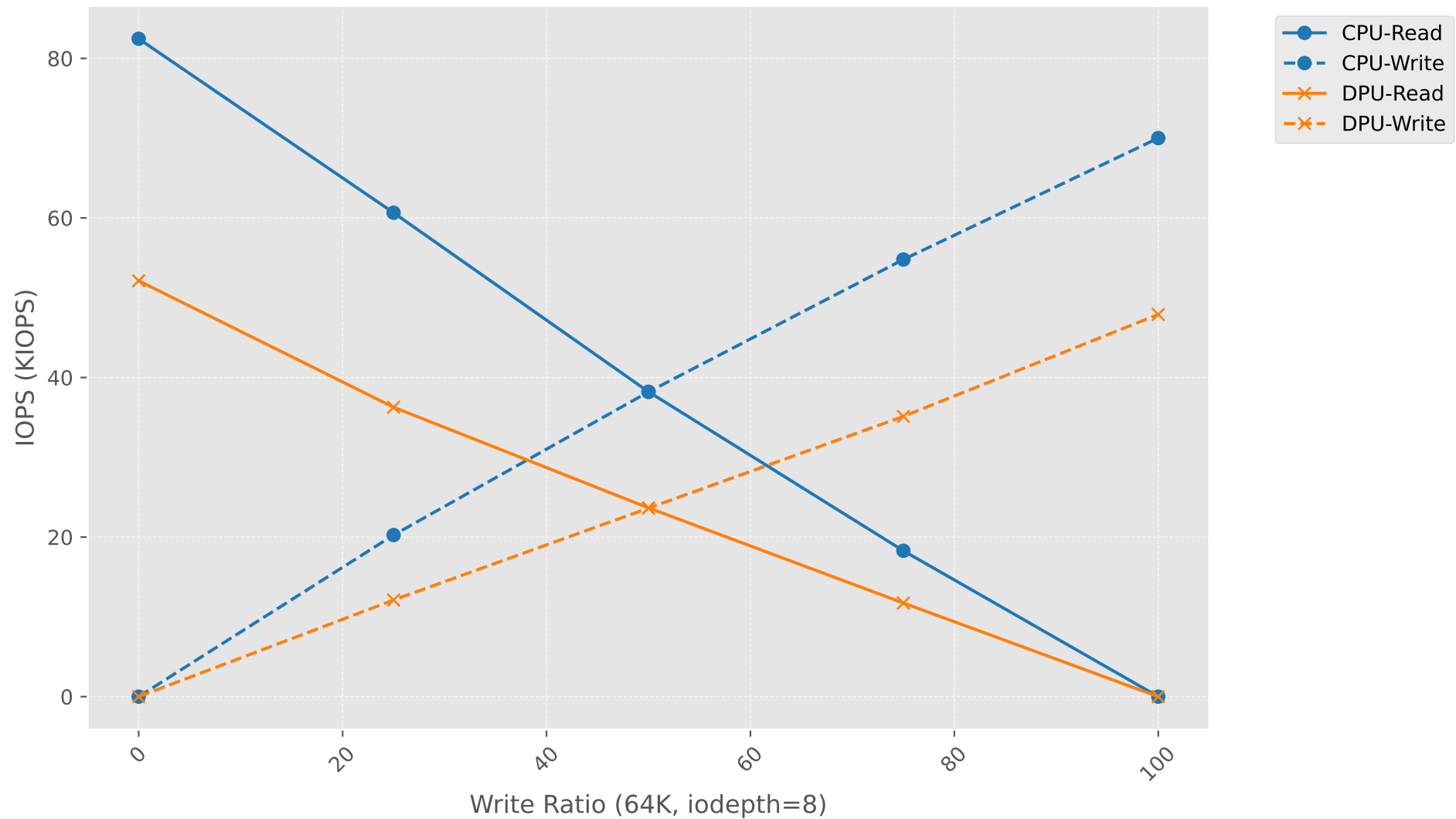
IOPS vs Write Ratio (64K, iodepth=8)
